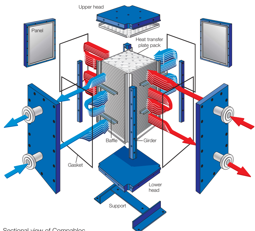
Sectional view of Compabloc
